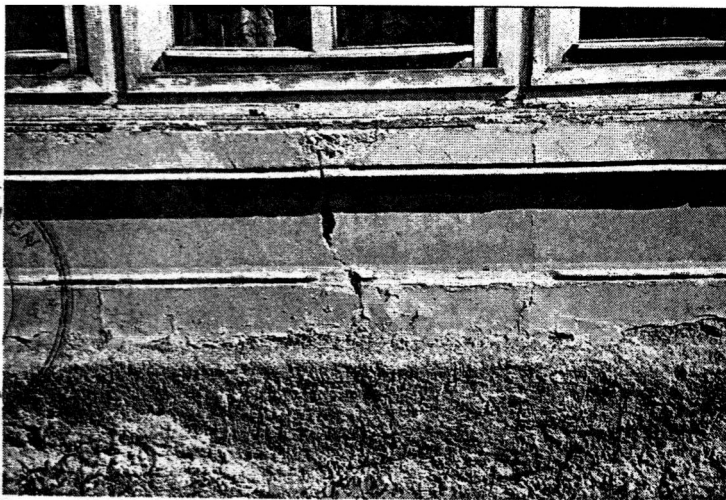
SOCLU FISURAT IN AXA 7
